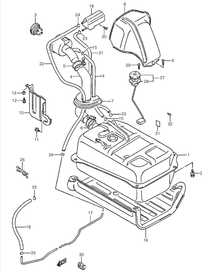
FIG. 93 FUEL TANK
