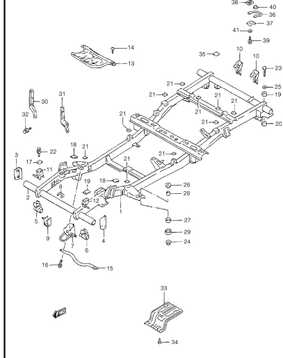
FIG. 64 CHASSIS FRAME
