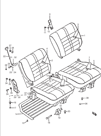
FIG. 95 REAR SEAT
