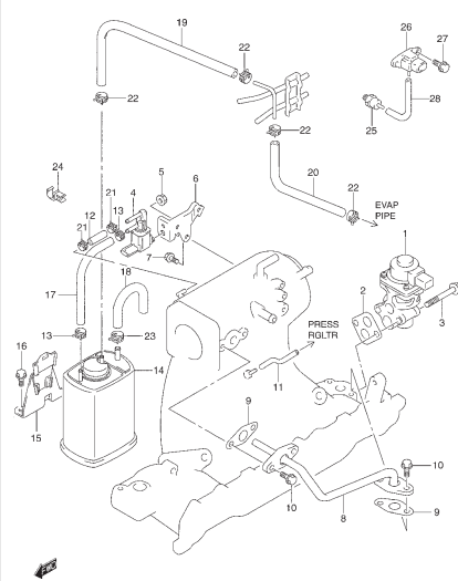
FIG. 21 EMISSION CONTROL
