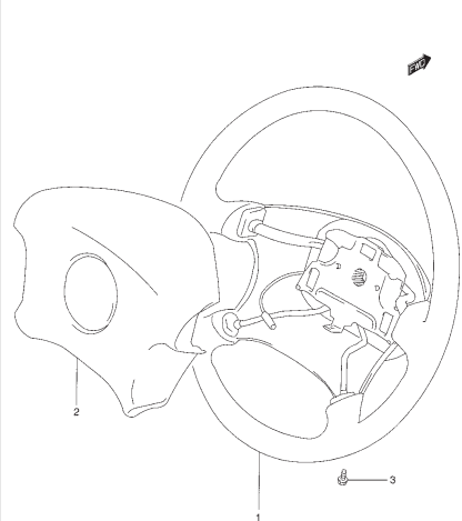
FIG. 53 STEERING WHEEL
