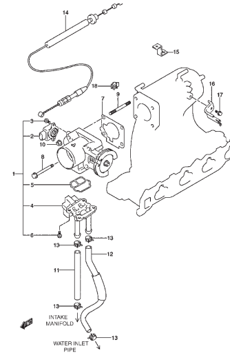
FIG. 12 THROTTLE BODY
