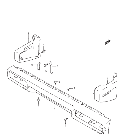
FIG. 75 REAR BUMPER
