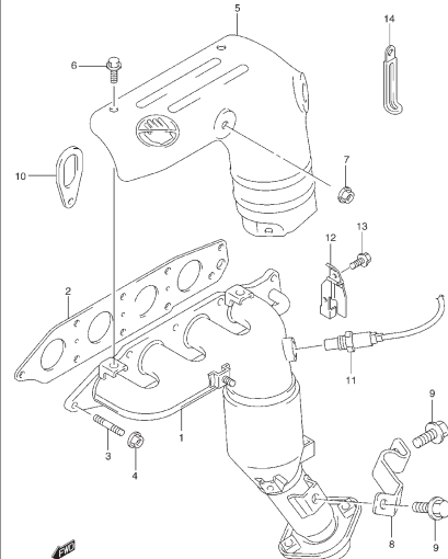
FIG. 15 EXHAUST MANIFOLD
