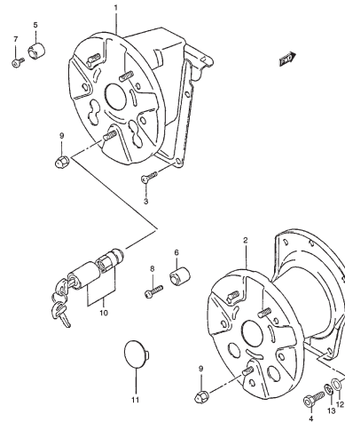
FIG. 82 TIRE CARRIER
