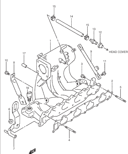
FIG. 11 INTAKE MANIFOLD
