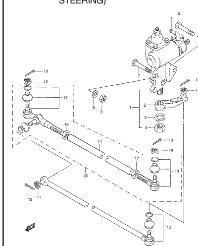
FIG. 56 STEERING LINK (W/ POWER STEERING)
