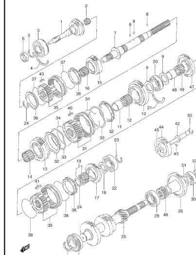
FIG. 24 TRANSMISSION
