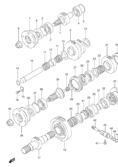
FIG. 31 TRANSFER GEAR
