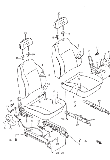
FIG. 94 FRONT SEAT
