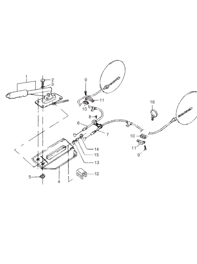
FIG. 63 PARKING BRAKE
