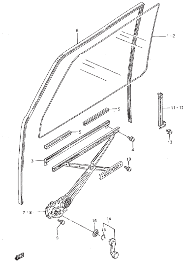
FIG. 87 FRONT DOOR REGULATOR
