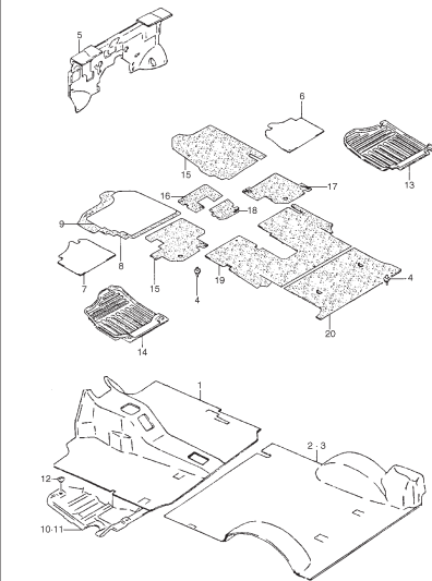
FIG. 79 FLOOR CARPET
