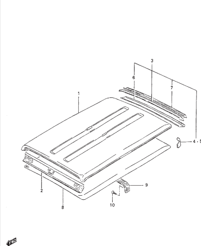
FIG. 73 ROOF PANEL (V)
