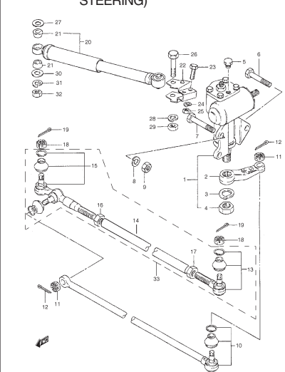
FIG. 55 STEERING LINK (N/ POWER STEERING)
