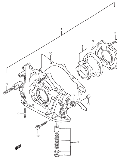
FIG. 6 OIL PUMP
