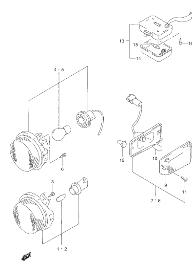
FIG. 40 FRONT LAMP AND ROOM LAMP
