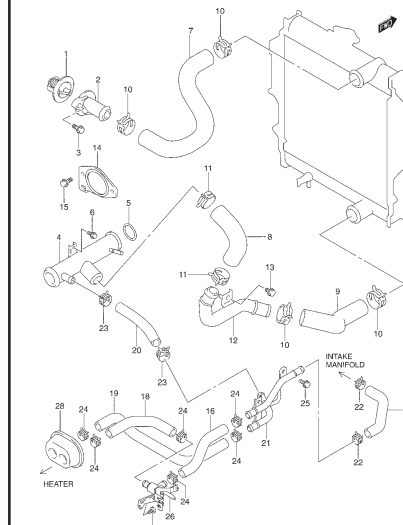
FIG. 20 WATER HOSE
