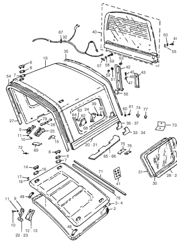
FIG. 85 HARD TOP ASSY
