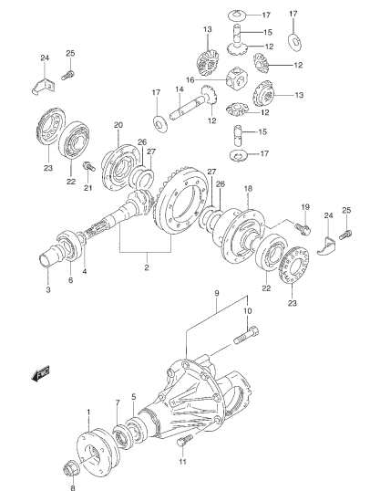
FIG. 30 REAR DIFF GEAR
