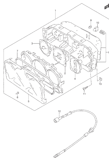
FIG. 38 INSTRUMENT PANEL
