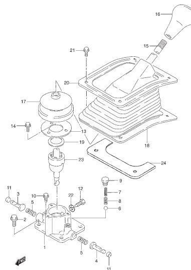
FIG. 31 TRANSFER GEAR
