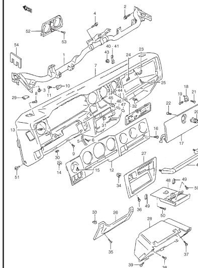
FIG. 80 INTERIOR TRIM
