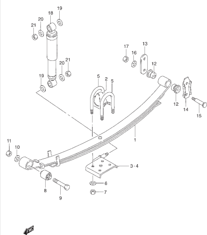
FIG. 49 REAR SUSPENSION
