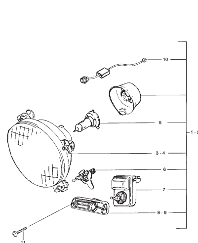
FIG. 39 HEAD LAMP
