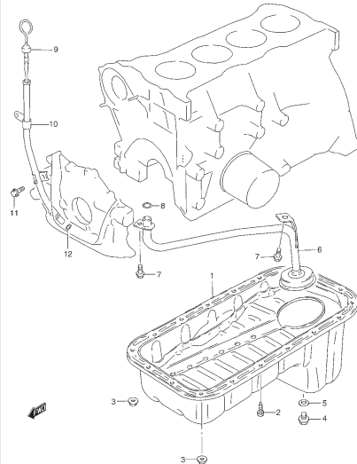
FIG. 5 OIL PAN
