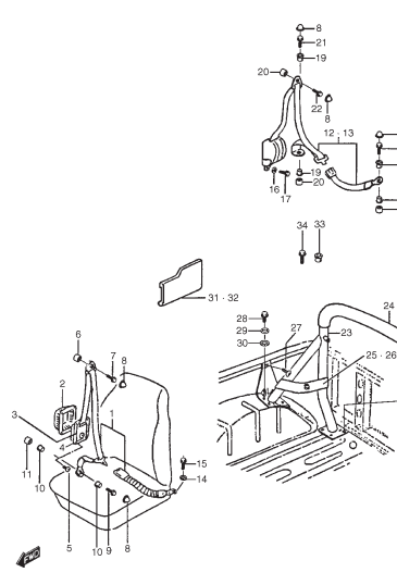
FIG. 96 SEAT BELTS
