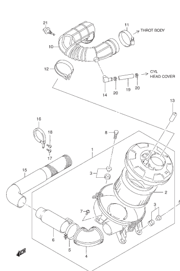
FIG. 14 AIR CLEANER
