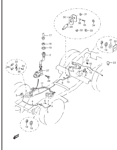
FIG. 64 CHASSIS FRAME
