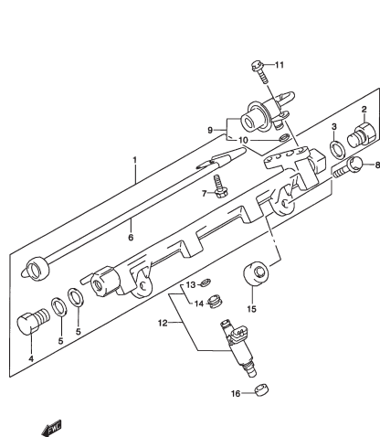
FIG. 13 DELIVERY PIPE
