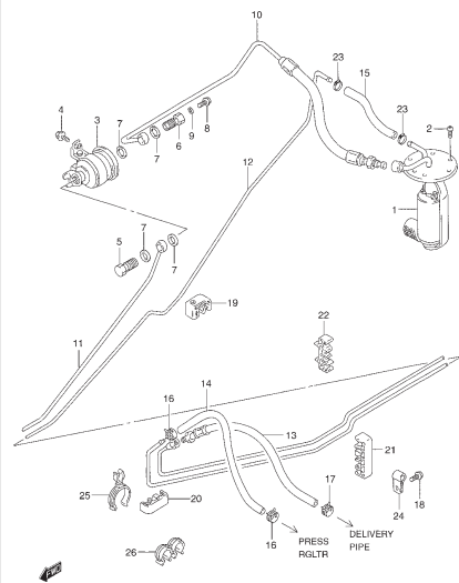
FIG. 17 FUEL PUMP
