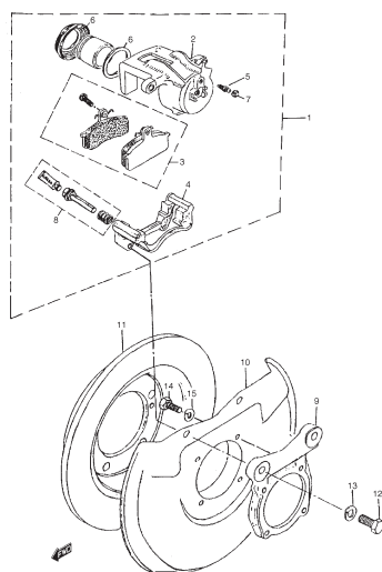
FIG. 61 FRONT WHEEL BRAKE
