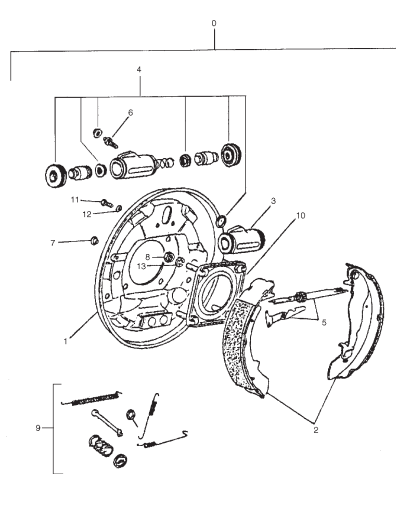
FIG. 62 REAR WHEEL BRAKE
