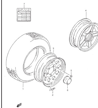
FIG. 52 TIRE / WHEEL
