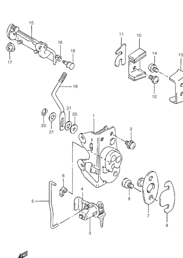
FIG. 95 REAR SEAT
