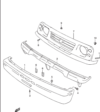
FIG. 74 FRONT BUMPER
