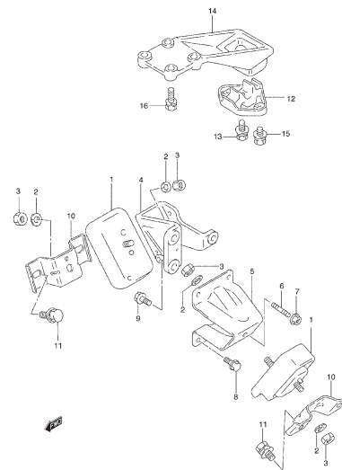
FIG. 7 ENGINE MOUNTING
