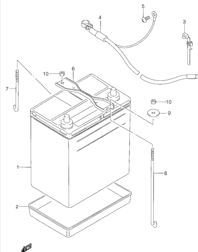
FIG. 37 BATTERY
